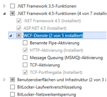
Abbildung 3: Features
